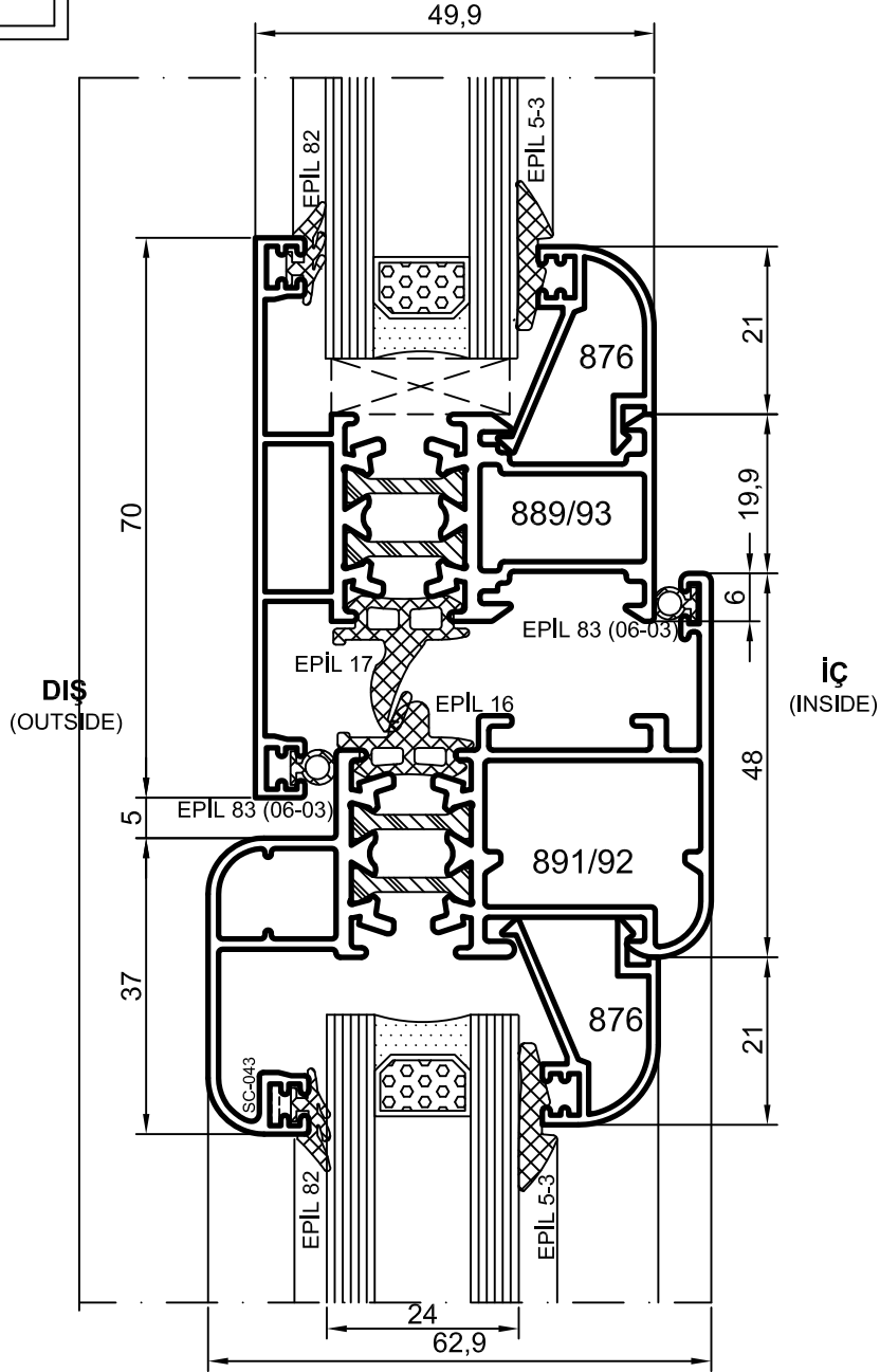
Detay Detail 6
