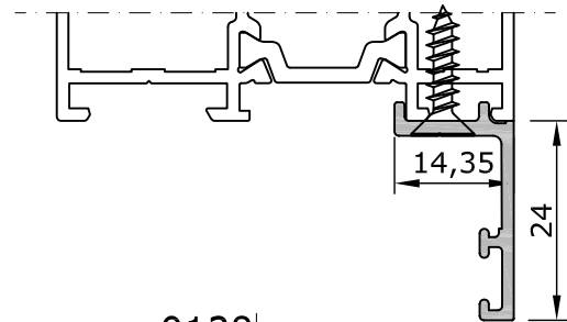
9138 Tırnak Profili 0,210 kg/m Cover Profile for PVC tilt and turn mechanism
