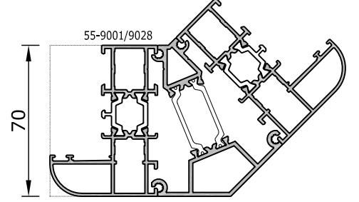
WT 70 P 1094 | 135 ° Dönüş Profili 1,415 kg/m | 135 ° Corner Profile J_x=20,05 \text{ cm}^4 | J_y=11,82 \text{ cm}^4
