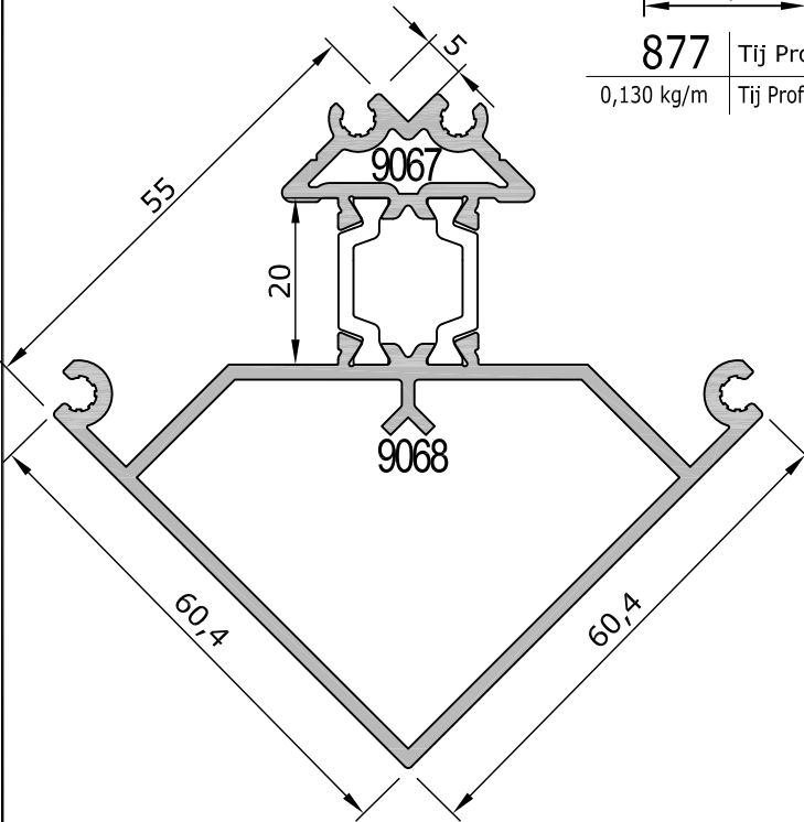
55-9067/9068 90 ° Dönüş Profili 1.790 kg/m | 90 ° Corner Profile Jx=26,96 cm 4 | Jy=25,71 cm 4
