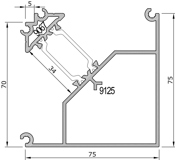
WT 70 P 1093 | 90 ° Dönüş Profili 2.015 kg/m | 90 ° Corner Profile J_x=35,83 \text{ cm}^4 | J_y=47,78 \text{ cm}^4
