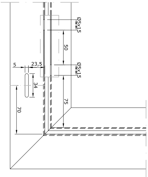
A DETAYI DETAIL A
