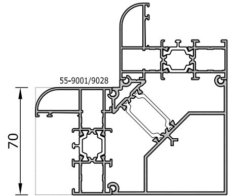
WT 70 P 1093 | 90 ° Dönüş Profili 2.015 kg/m | 90 ° Corner Profile J_x=35,83 \text{ cm}^4 | J_y=47,78 \text{ cm}^4
