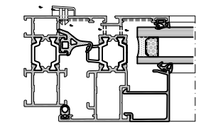
A DETAYI DETAIL A
