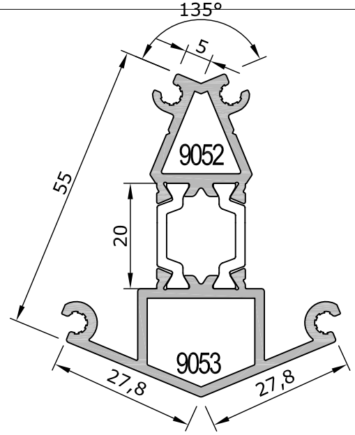
55-9052/9053 135 ° Dönüş Profili 1,305 kg/m | 135 ° Corner Profile Jx=14,79 cm 4 | Jy=5,64 cm 4
